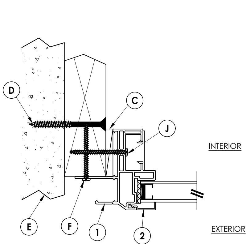
1 2 HORIZONTAL CROSS SECTION 2X BUCK MASONRY CONSTRUCTION
