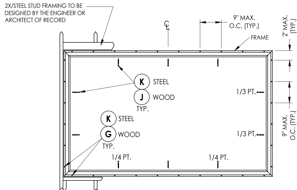
FRAME ANCHORING (STUD CONSTRUCTION)
