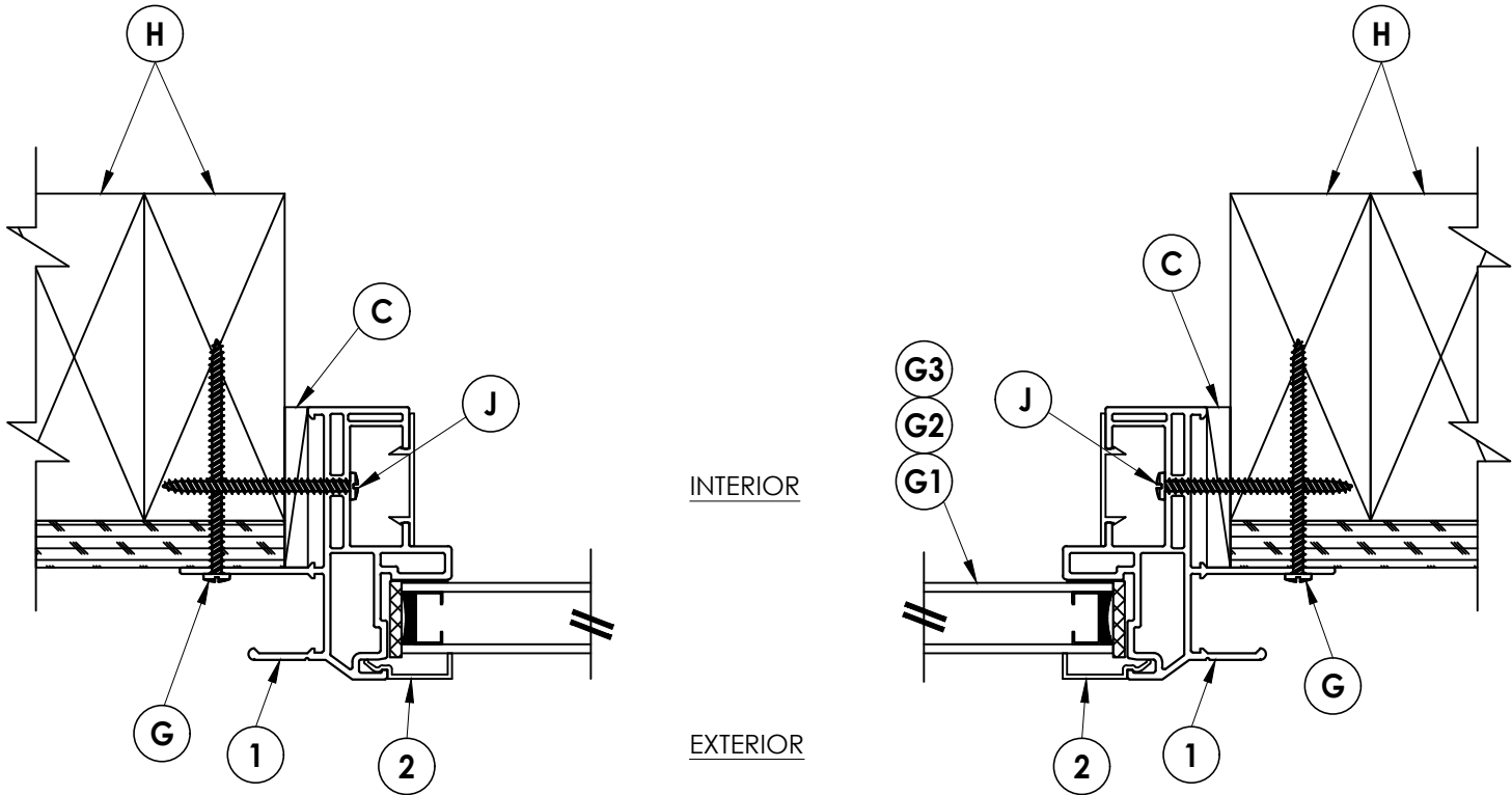
1 3 HORIZONTAL CROSS SECTION
