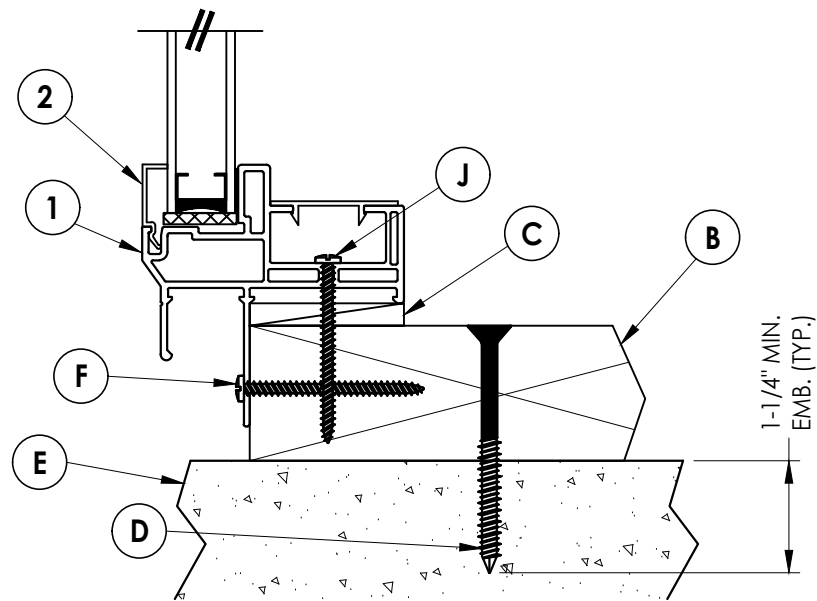
2 2 VERTICAL CROSS SECTION 2X BUCK MASONRY CONSTRUCTION
