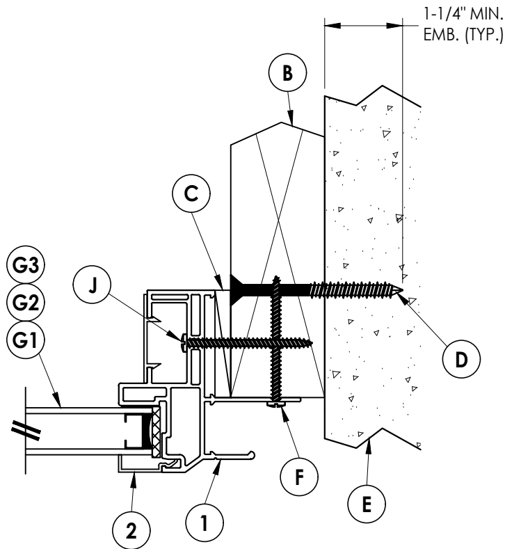
1 2 HORIZONTAL CROSS SECTION 2X BUCK MASONRY CONSTRUCTION
