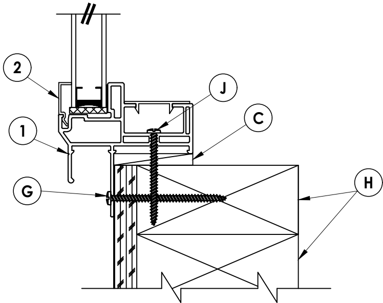
2 3 VERTICAL CROSS SECTION
