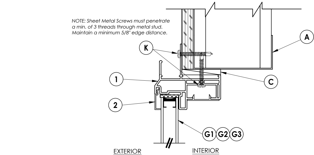
3 3 VERTICAL CROSS SECTION Shown w/ Steel Stud Framing Option
